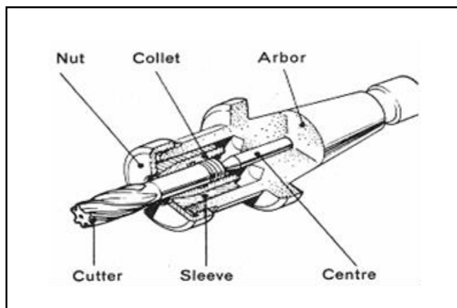
Figure 3.1: Parts of an arbor with nut is clearly shown together with the milling tool attached for the use of pneumatic clamping on CNC machine (Hasley 2007).
